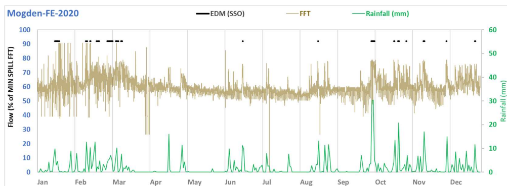
Figure 2: individual spills from Mogden STW in 2020 ( black segments ); during spills, the flow to full treatment ( brown curve ) should be above 92% capacity (8% meter error is allowed); all of the spills are illegal
