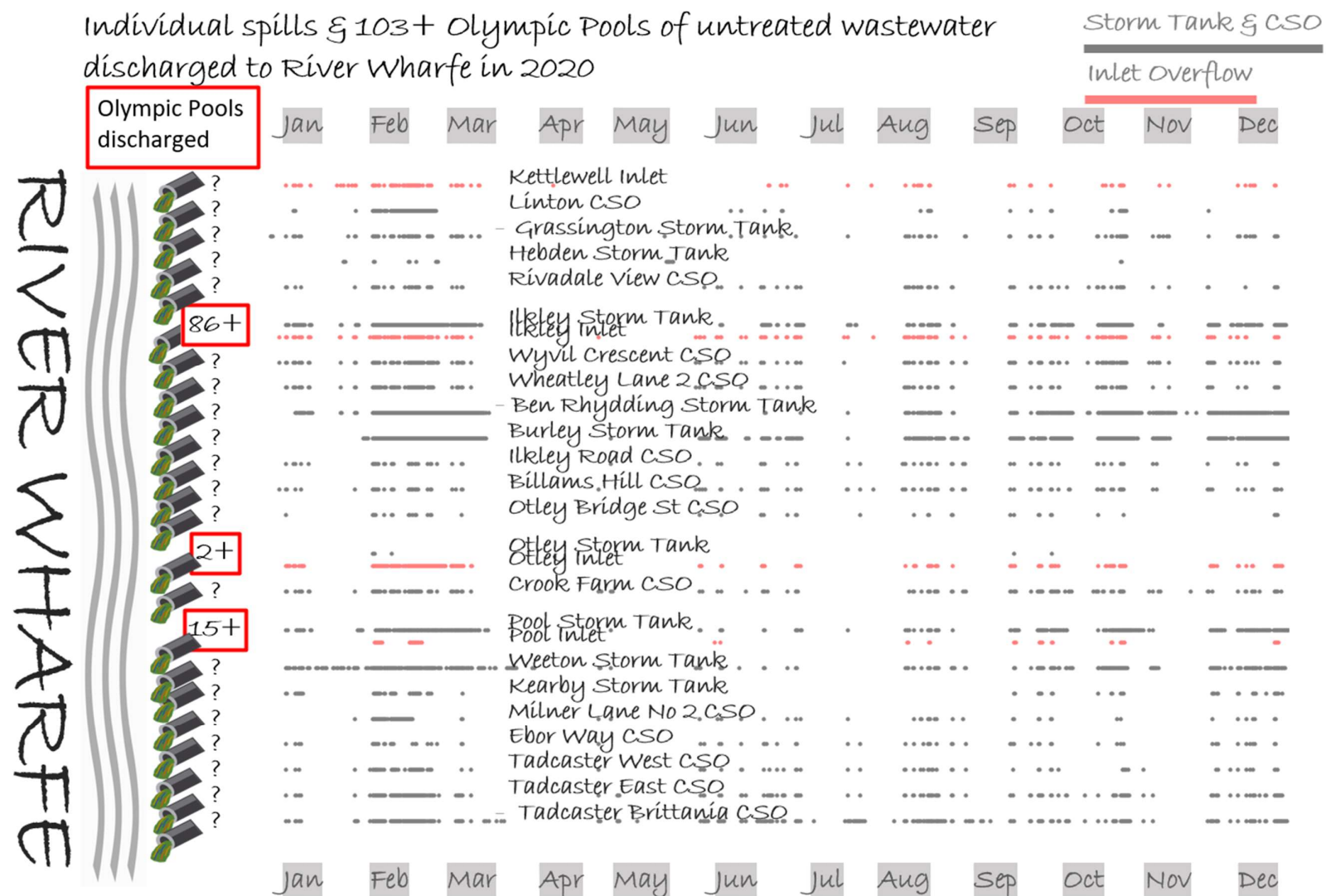
Figure 9: individual spills in 2020 to the River Wharfe via 4 STW inlets (pink segments), 13 CSOs and 9 storm tank overflows (grey segments) The 26 storm overflows spilled for a total of 17,775 hours, but the volume of discharge can be estimated for only 3 – the estimates are for a minimum value only
